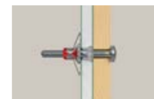
One plug length covers all common building material thicknesses from 9.5 - 30 mm, for flexible and cost-efficient application.
